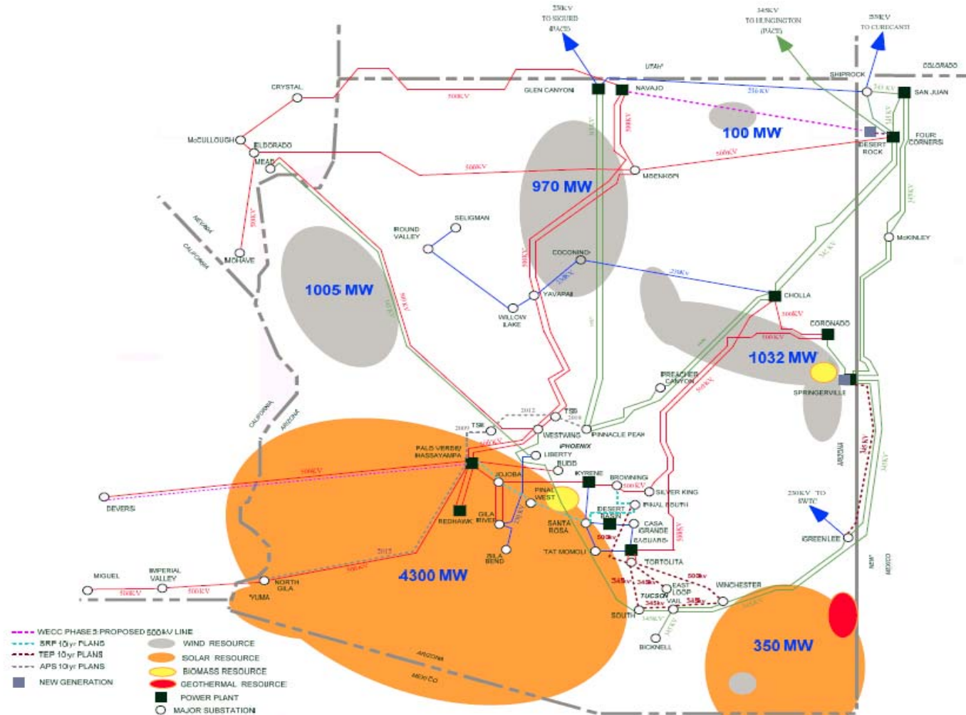
Figure 2: Potential Arizona Renewable Resources
